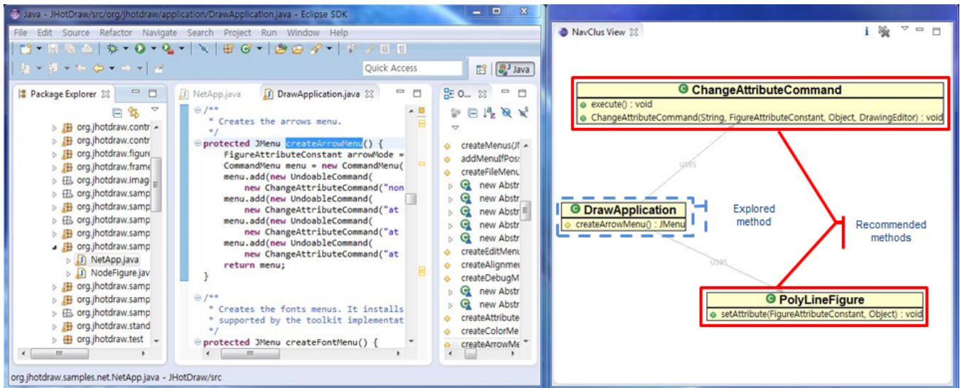
Fig. 1. NavClus User Interface
